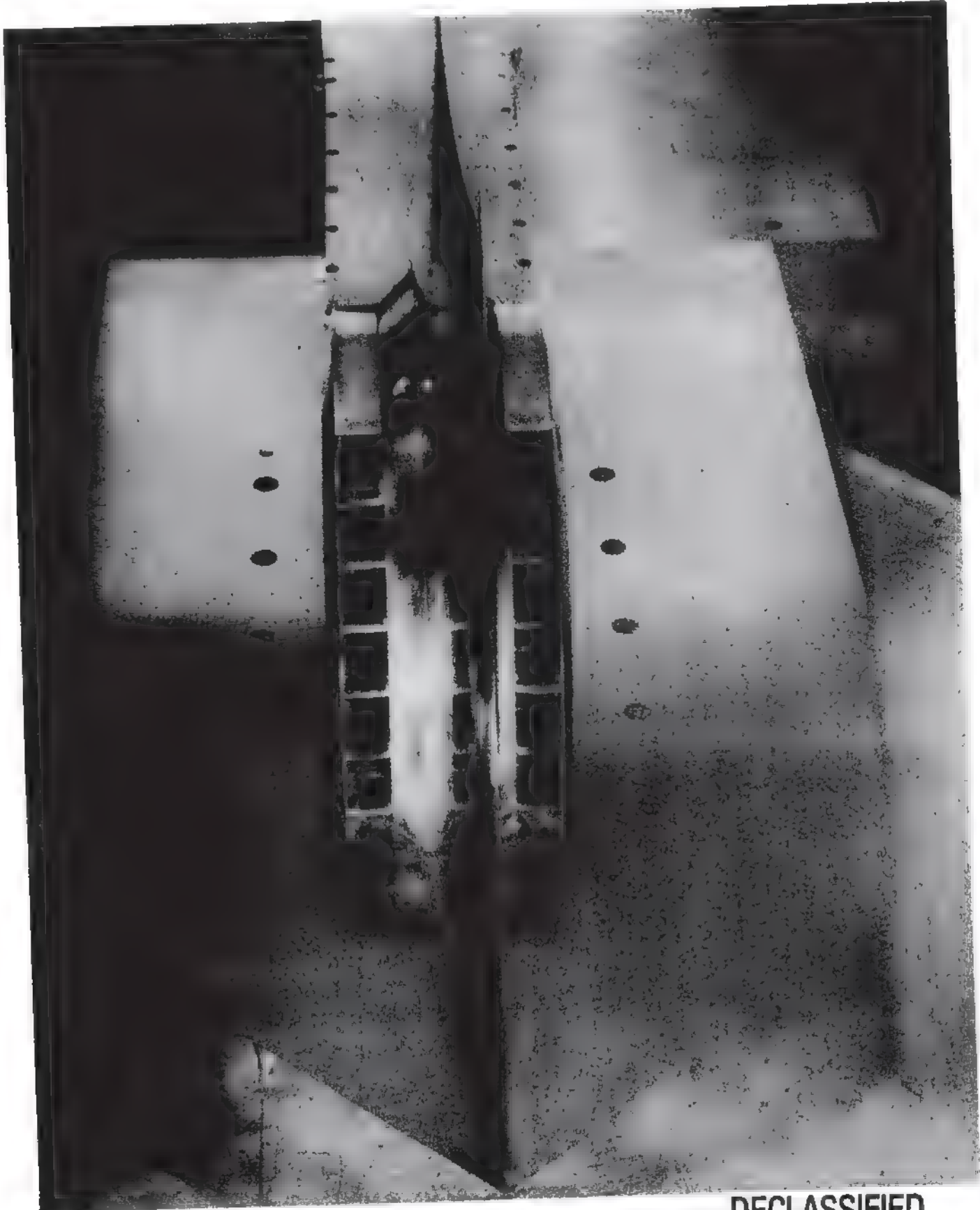
FIG. 15 2/25 SCALE AIR INTAKE MODEL DECLASSIFIED
